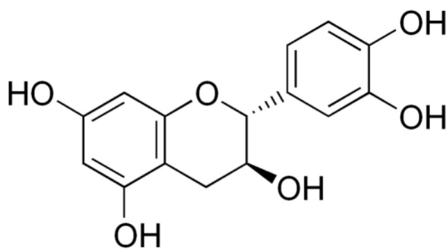
Catechin
